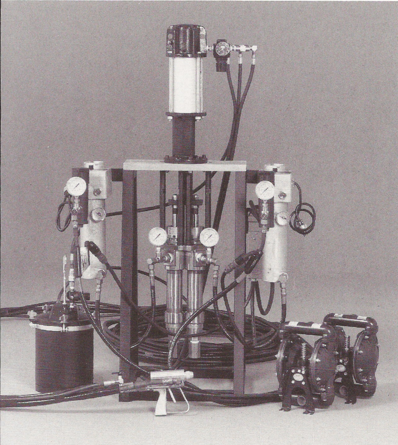
HEATED SYSTEM WITH TRANSFER PUMPS
