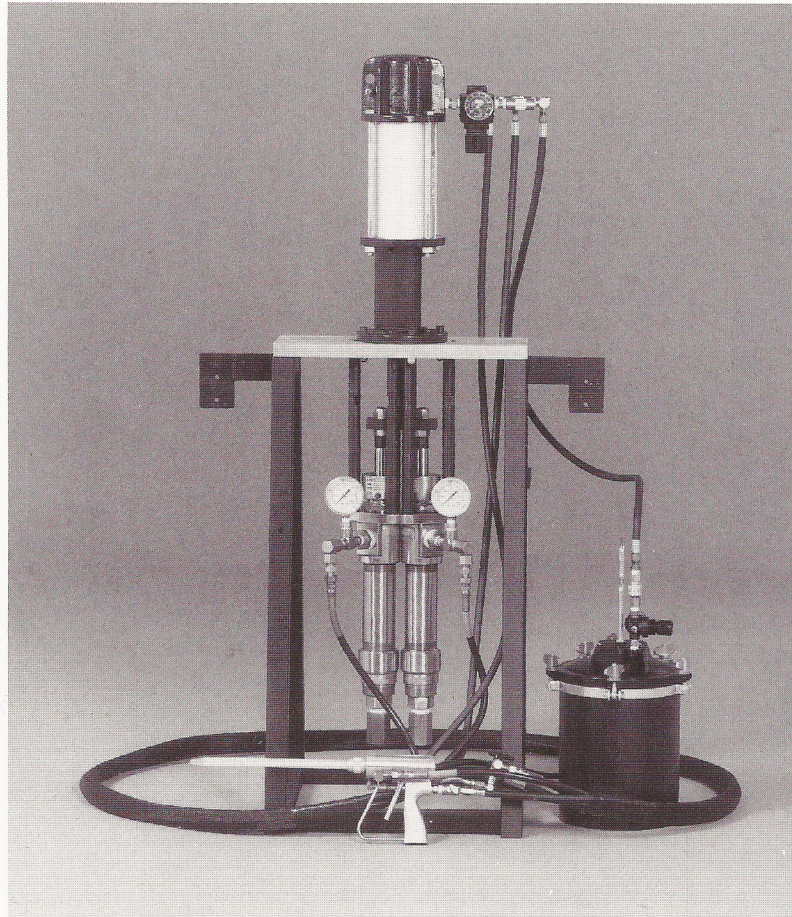
STANDARD SYSTEM
